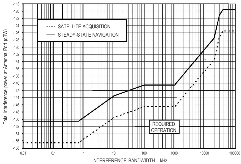
Figure B-37. Interference thresholds versus bandwidth for GPS L1 and SBAS L1 receivers
