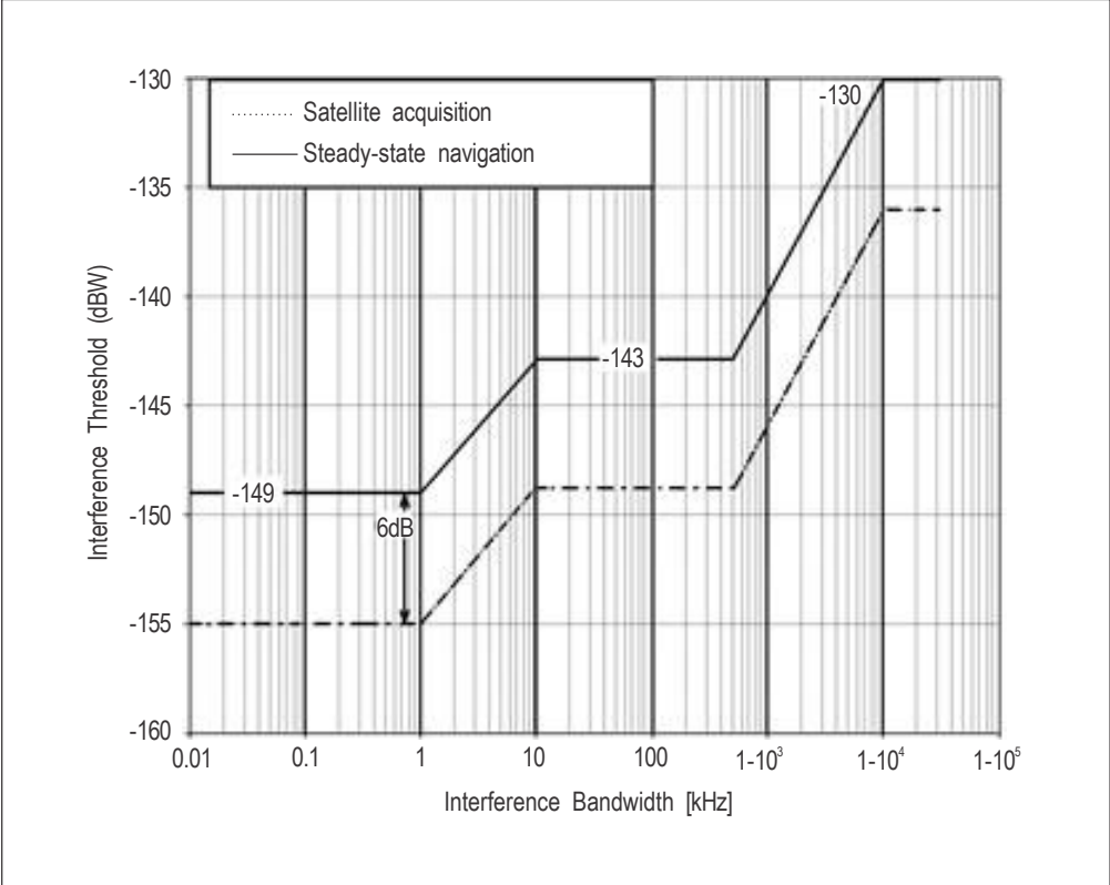
Figure B-38. Interference thresholds versus bandwidth for GLONASS FDMA signals receivers in L1 band
