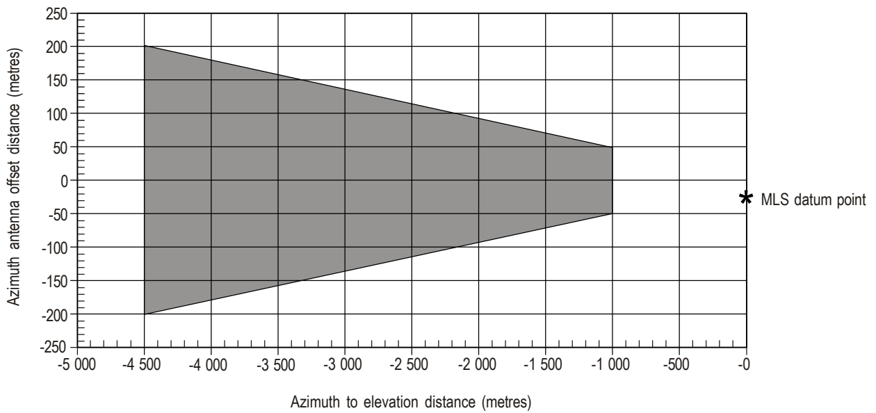
Figure G-31. Permissible azimuth antenna offsets for computed centre line approaches with DME/N ranging
