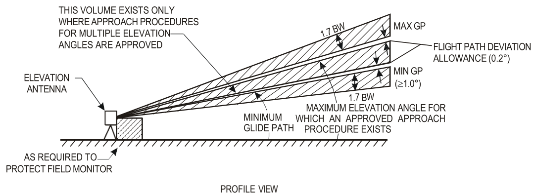
Figure G-24. Typical elevation critical and sensitive areas/volume
