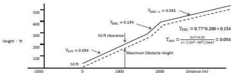
Figure 3: Assumed engine failure height less than 200 ft
