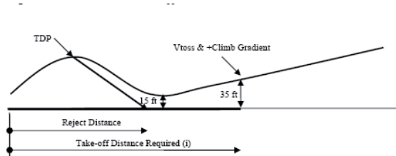
Figure 1: Clear Area take – off
