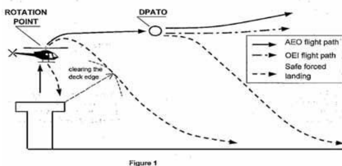
Figure 1: Typical take-off profile PC2 from a helideck/elevated FATO, non-hostile environment
