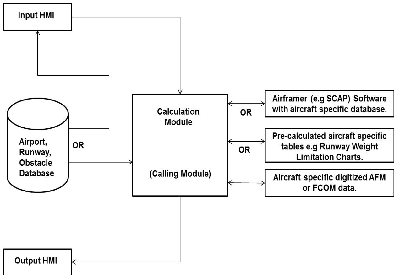
Figure 1. Typical architecture of a performance application
