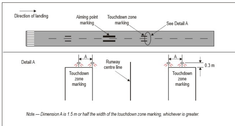
Figure 23 - Simple touchdown zone lighting
