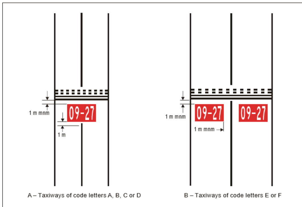
Figure 10 - Mandatory instruction marking
