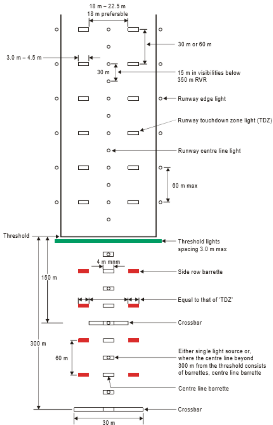
Figure 15 - Inner 300 m approach and runway lighting for precision approach runways, categories II and III, where the serviceability levels of the lights specified as maintenance objectives in SD-AD appendix 10 can be demonstrated
