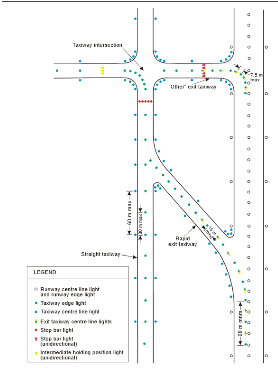
Figure 25 - Taxiway lighting
