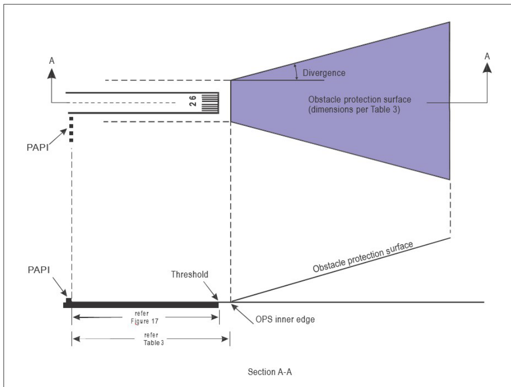
Figure 19 - Obstacle protection surface for visual approach slope indicator systems
