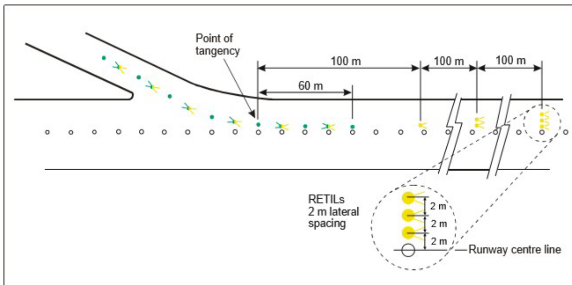
Figure 24- Rapid exit taxiway indicator lights (RETILs)
