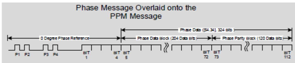
Figure 3-10. Phase overlay message structure
