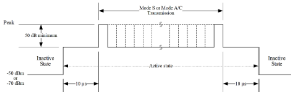
Figure 3-11 Unwanted output power
