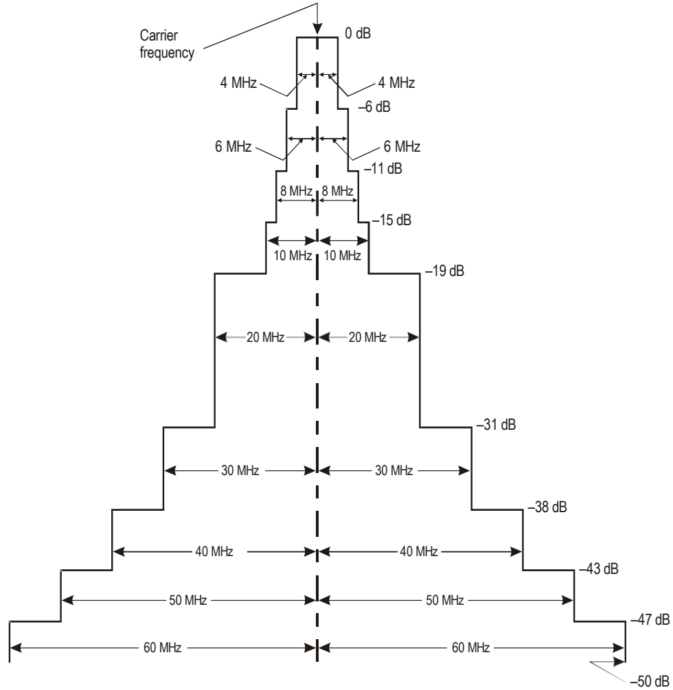
Figure 3-2. Required spectrum limits for interrogator transmitter
