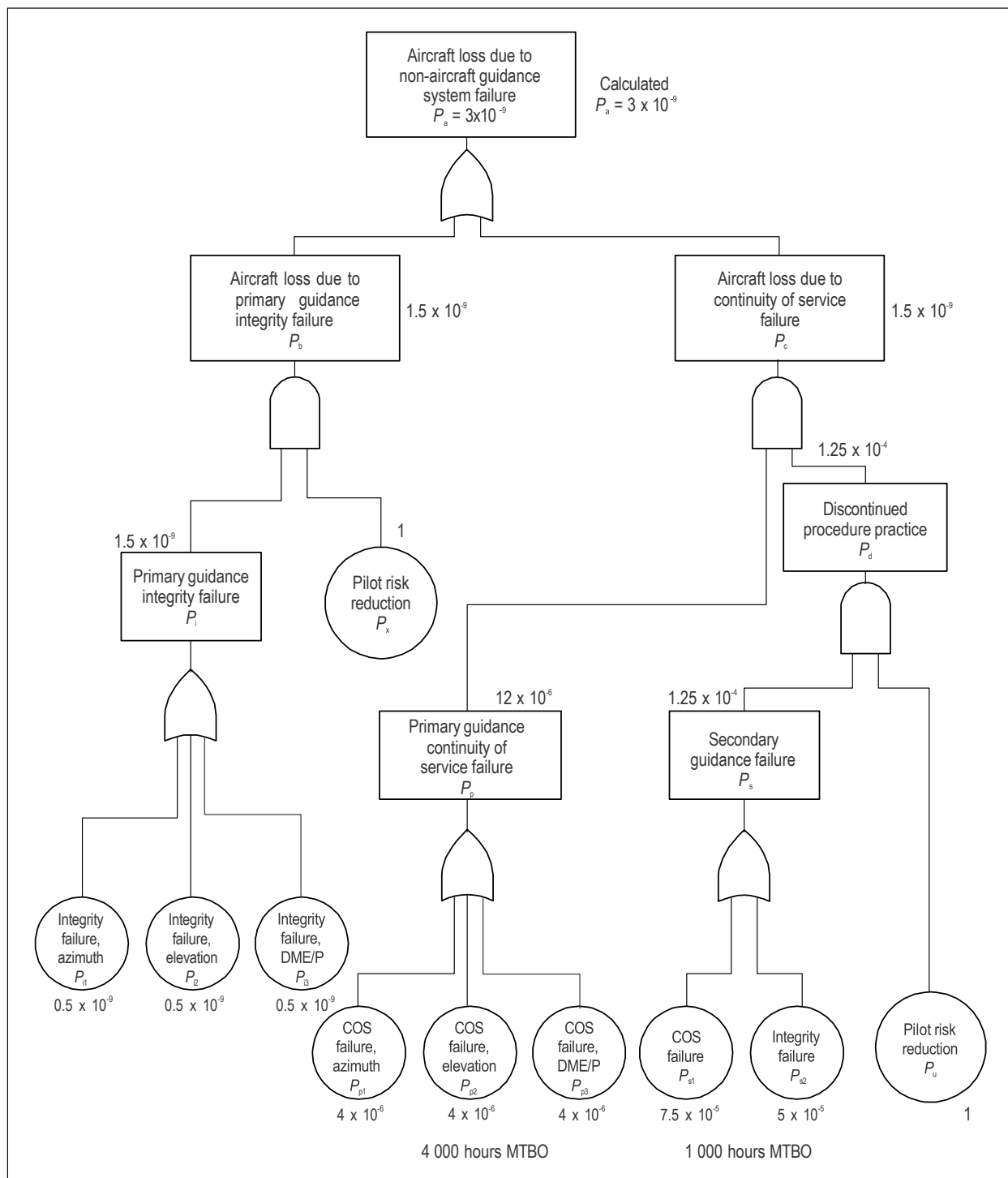
Figure A-3. MLS/ area navigation RNAV obstacle rich risk tree
