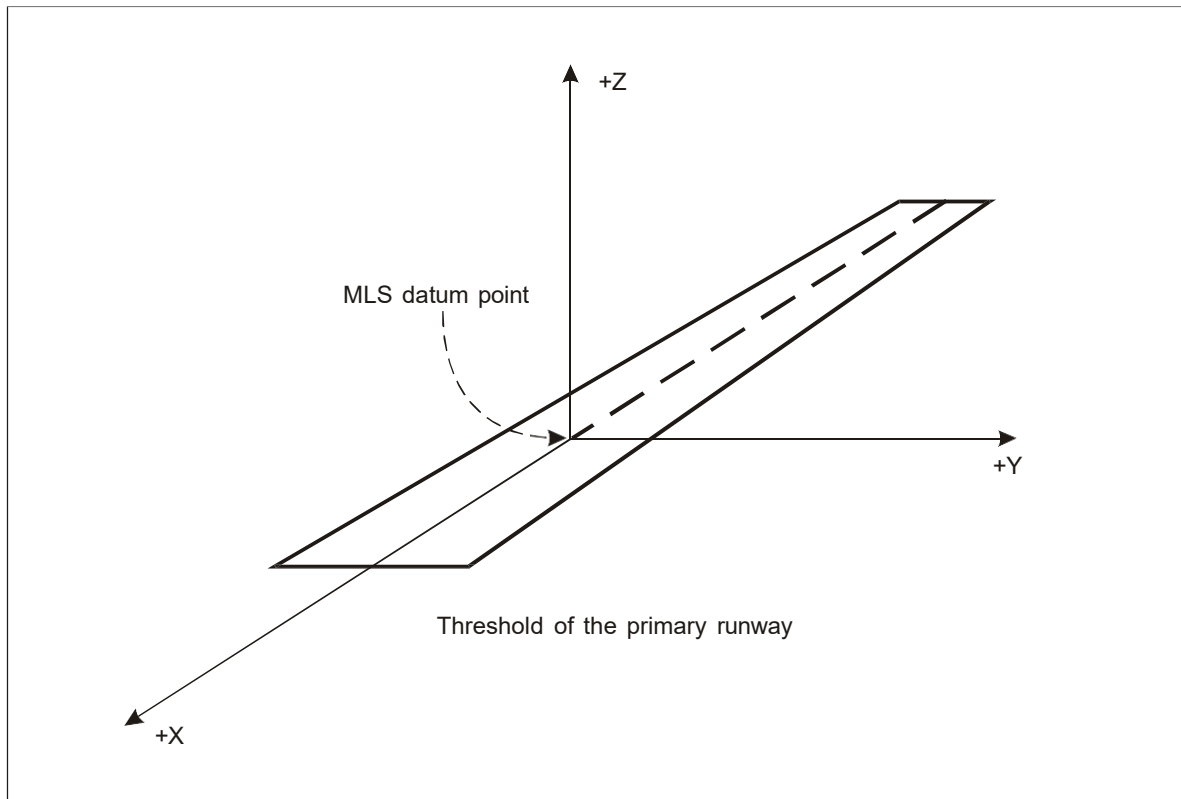
Figure G-13. MLS/ area navigation RNP-V way-point coordinate system
