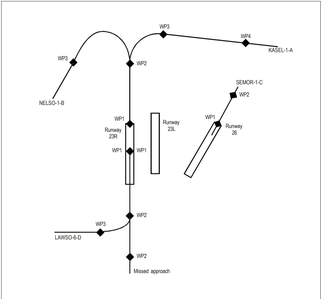
Figure G-15. Diagram of sample MLS/ area navigation RNAV procedures
